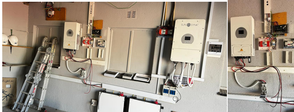
Solar PV installation for showcase/teaching purposes and a training inverter stations.
